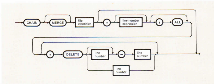
Figure 11-1 CHAIN Statement
