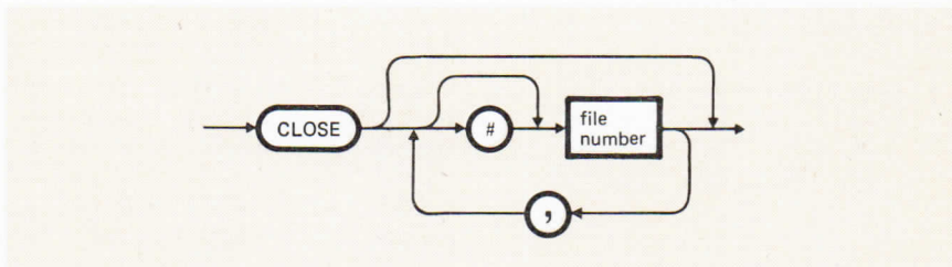
Figure 12-2 CLOSE Statement
