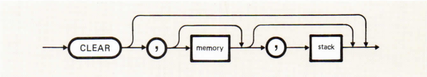
Figure 5-1 CLEAR Statement
