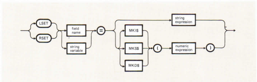
Figure 12-11 LSET/RSET Statements
