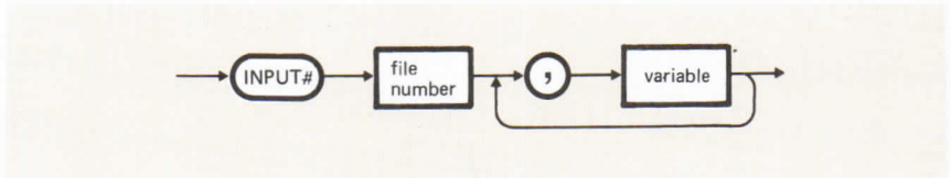
Figure 12-7 INPUT# Statement
