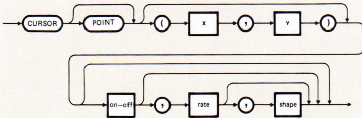
Figure 14-18 CURSOR Statement
