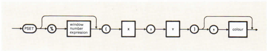
Figure 14-15 PSET Statement
