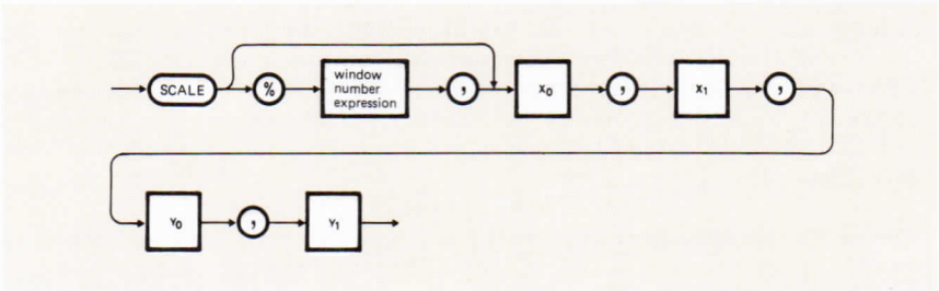
Figure 14-10 SCALE Statement
