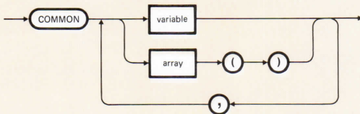
Figure 11-2 COMMON Statement
