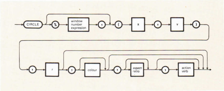
Figure 14-22 CIRCLE Statement
