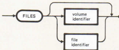
Figure 3-7 FILES Command
