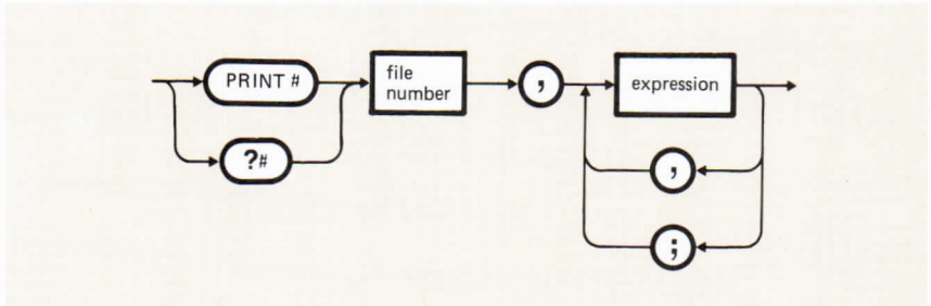
Figure 12-3 PRINT# Statement:
