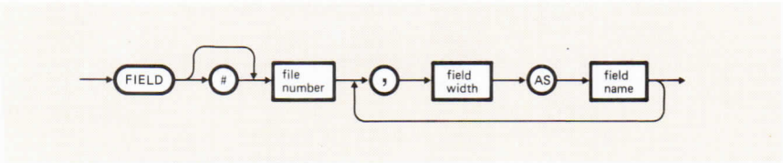
Figure 12-10 FIELD Statement
