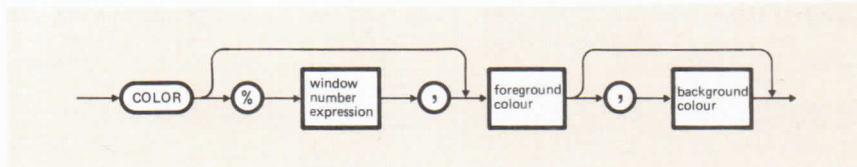
Figure 14-8 COLOR Statement
