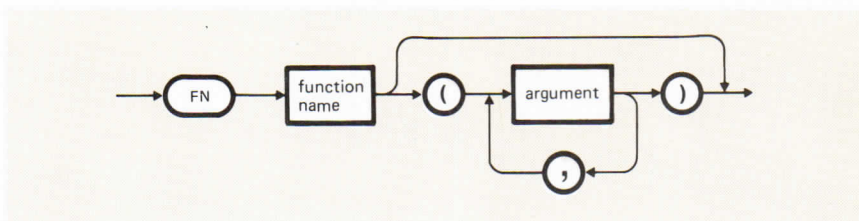
Figure 9-2 Function Call
