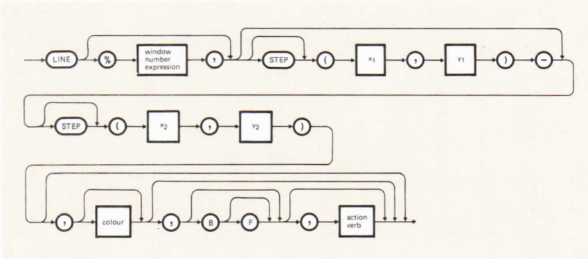
Figure 14-20 LINE Statement
