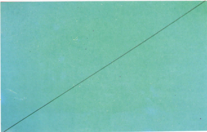
Figure 14-11 LINE Statement
