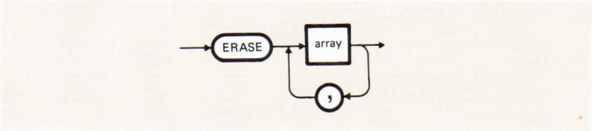
Figure 4-3 ERASE Statement
