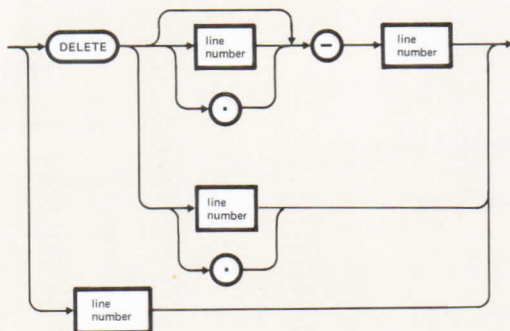
Figure 3-1 DELETE Command
