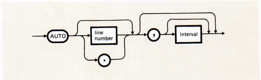
Figure 2-3 AUTO Command
