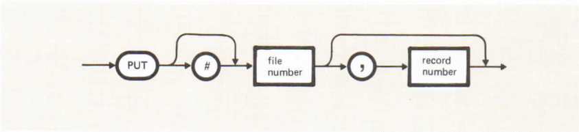
Figure 12-15 PUT-File Statement
