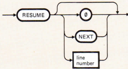
Figure 13-10 RESUME Statement
