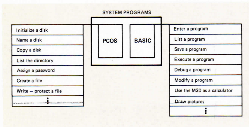
Figure 1-1 System Programs
