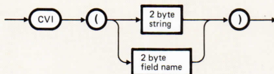
Figure 12-18 CVI Function
