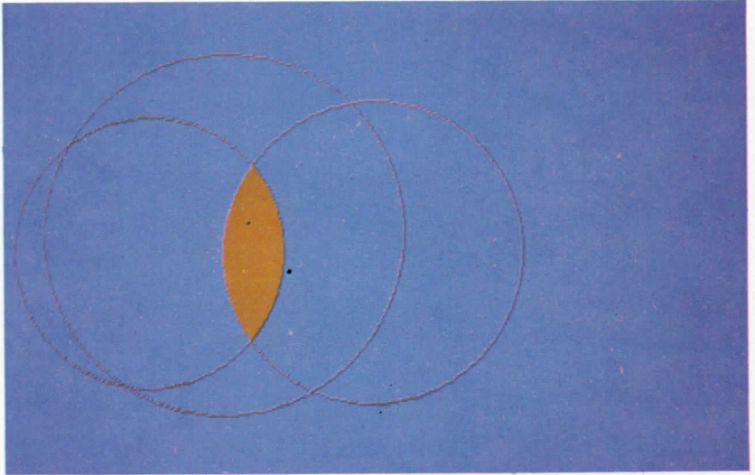
Figure 14-23 Intersecting Circles
