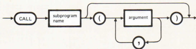
Figure 10-5 CALL Statement
