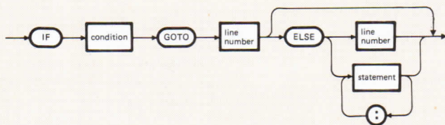
Figure 8-3 IF...GOTO...ELSE Statement
