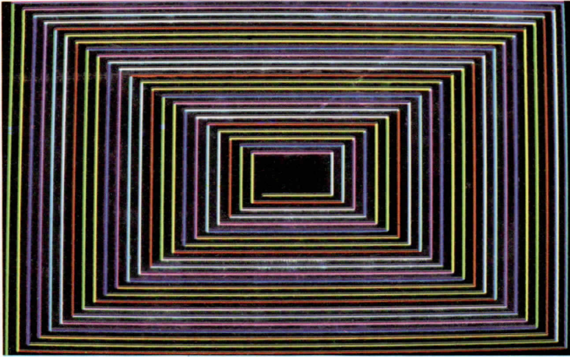
Figure 14-25
