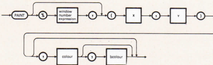
Figure 14-26 PAINT Statement
