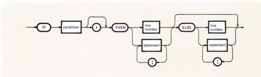
Figure 8-4 IF...THEN...ELSE Statement
