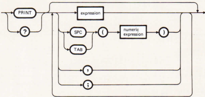
Figure 7-4 PRINT Statement
