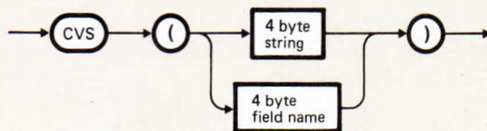
Figure 12-19 CVS Function
