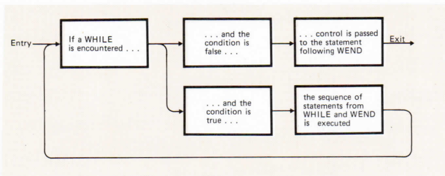
Figure 8-10 WHILE/WEND Statements
