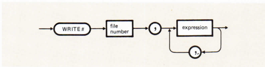
Figure 12-5 WRITE# Statement
