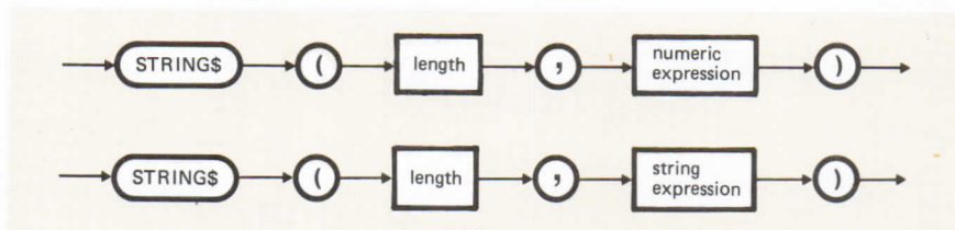
Figure 9-34 STRING$ Function
