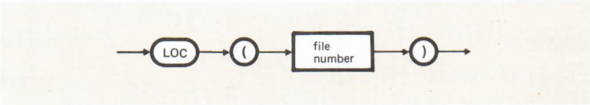
Figure 12-16 LOC Function
