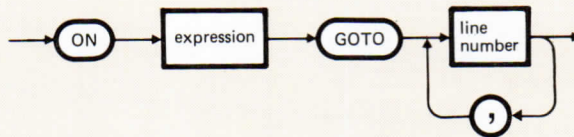
Figure 8-2 ON...GOTO Statement
