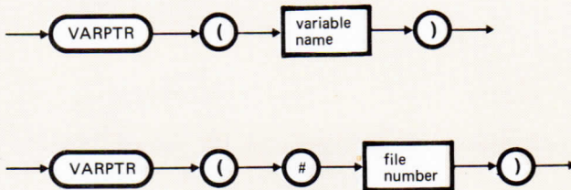
Figure 9-4 VARPTR Function
